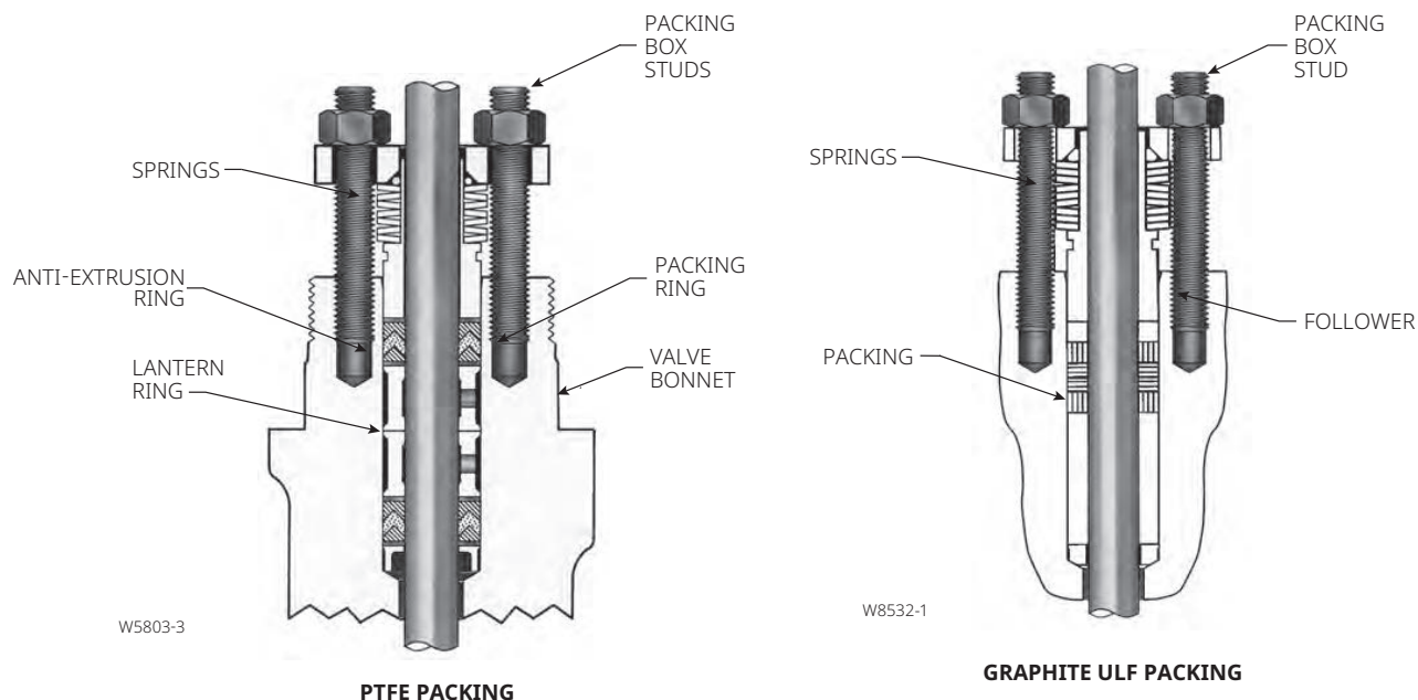
Figure 6. ENVIRO-SEAL Packing Systems
