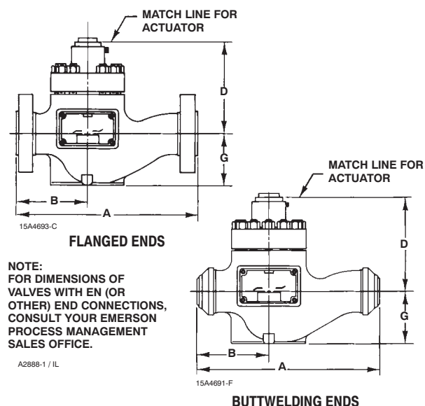
Figure 31. Dimensions (NPS 8 through 14 Fisher® EHD and EHT Valves) (also see tables 29 and 30)
