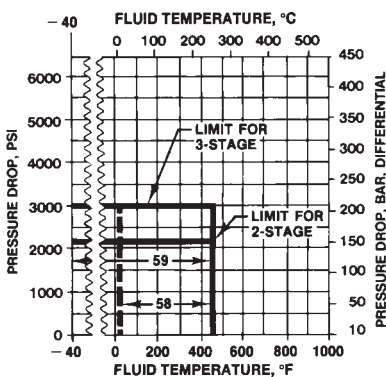
O-RING CONSTRUCTION ONLY
