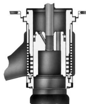
Figure 10. Fisher® EHAT Trim (NPS 3 through 8 Angle Valves)
