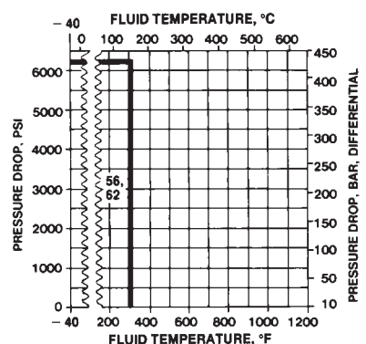
O-RING CONSTRUCTION ONLY (SOUR SERVICE)
