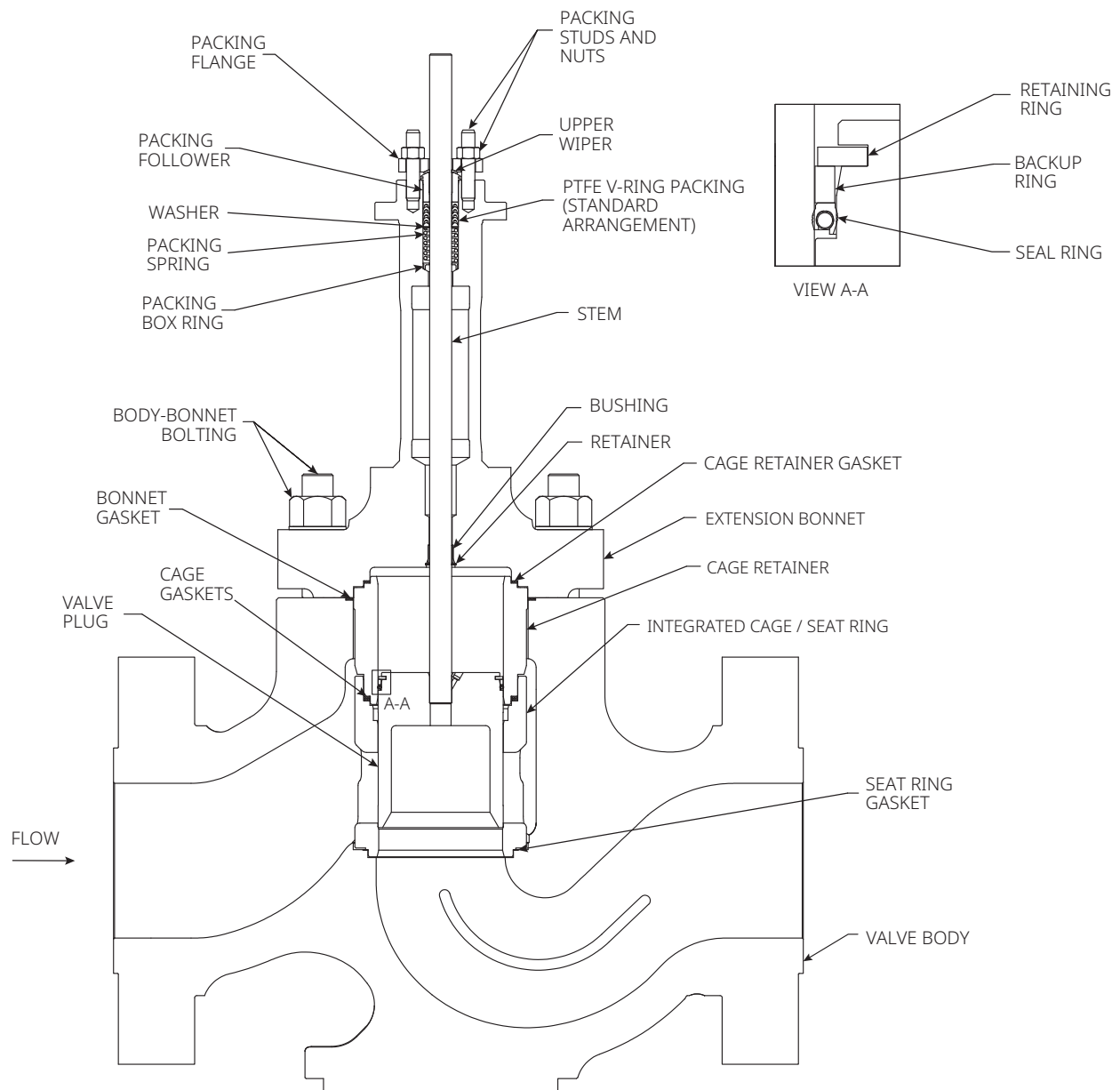
Figure 4. Fisher HPT-C Valve Assembly Detail with Fabricated Extension Bonnet NPS 8 through 12 (Long)
