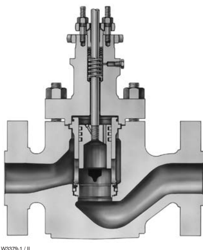
Figure 5. Fisher® EHD Valve Body Assembly
