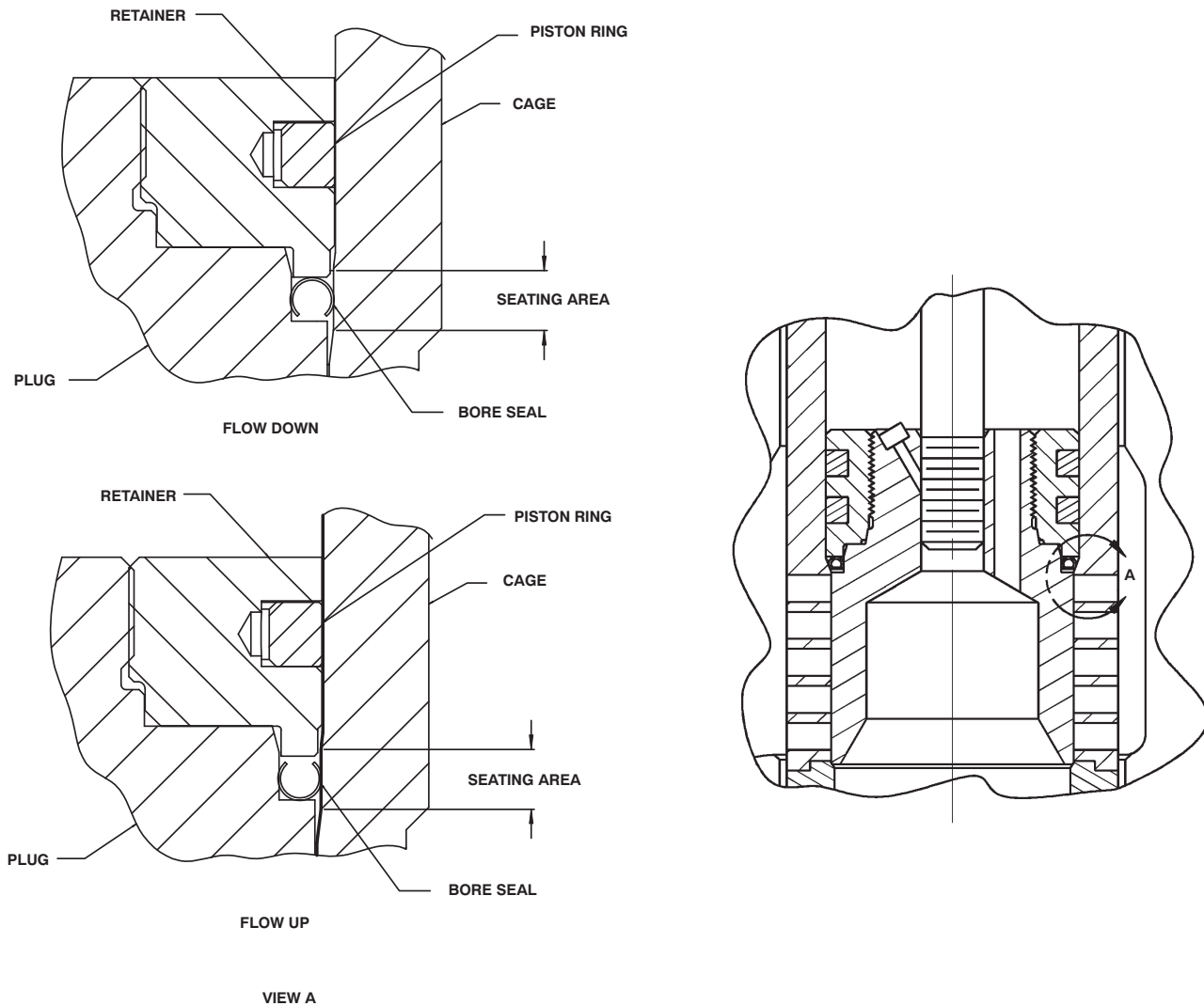
Figure 22. Bore Seal Trim
