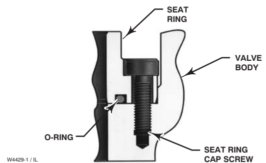
O-RING GASKET CONSTRUCTION (STANDARD CONSTRUCTION FOR SOUR SERVICE AND OPTIONAL FOR OTHER VALVE CONSTRUCTIONS)
