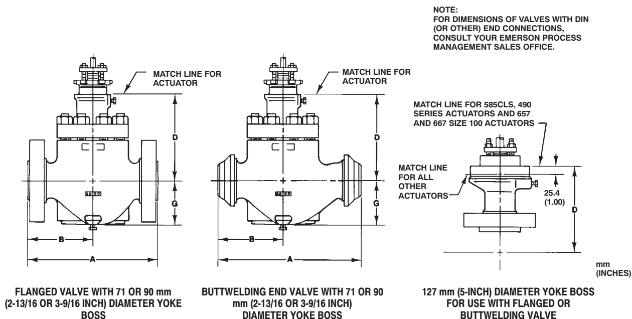
Figure 28. NPS 1-1/2 x 1 through 6 Globe Valve Dimensions with Standard Bonnet (also see tables 24, 25, and 26)
