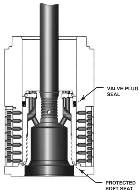
Figure 23. Typical Balanced TSO (Tight Shutoff) Trim
