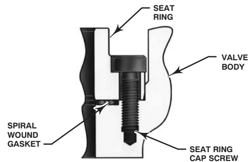
SPIRAL WOUND GASKET CONSTRUCTION (STANDARD CONSTRUCTION)
