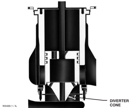
DIVERTER CONE VALVE PLUG USED IN BOILER FEEDWATER SERVICE FOR \Delta P > 1000 PSI (69 BAR) AND IN OTHER APPLICATIONS FOR \Delta P > 2000 PSI (138 BAR) OR FOR WHISPER TRIM III LEVEL A, B, OR C CAGES
