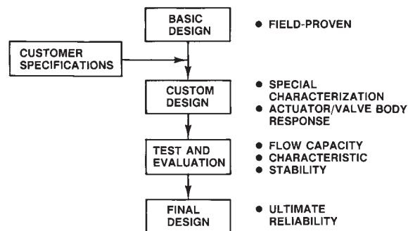
Figure 20. Custom Design Sequence (NPS 20 Globe Valves)
