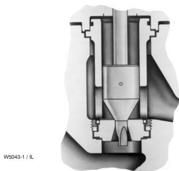
Figure 7. Fisher® EHS Trim with Micro-Flute Valve Plug
