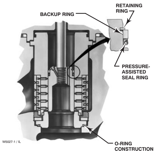
Figure 8. Fisher® EHT Trim w/ Cavitrol® III Three-Stage Cage
